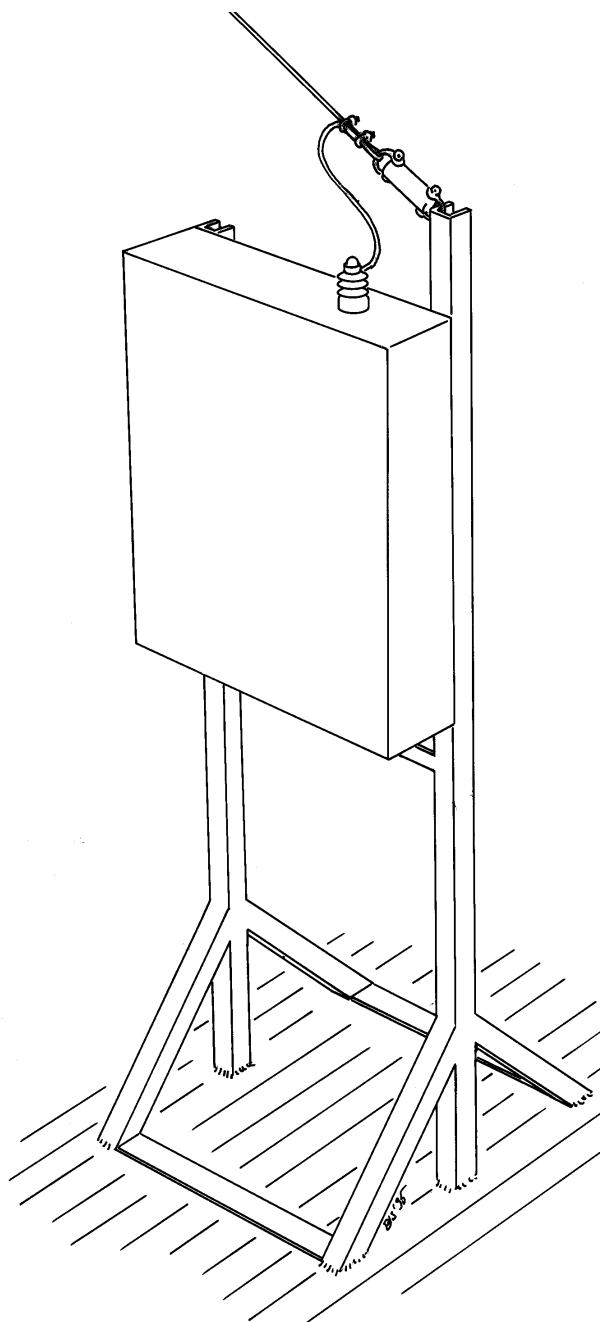
Antenna Tuning Unit bracket welded to the floor
