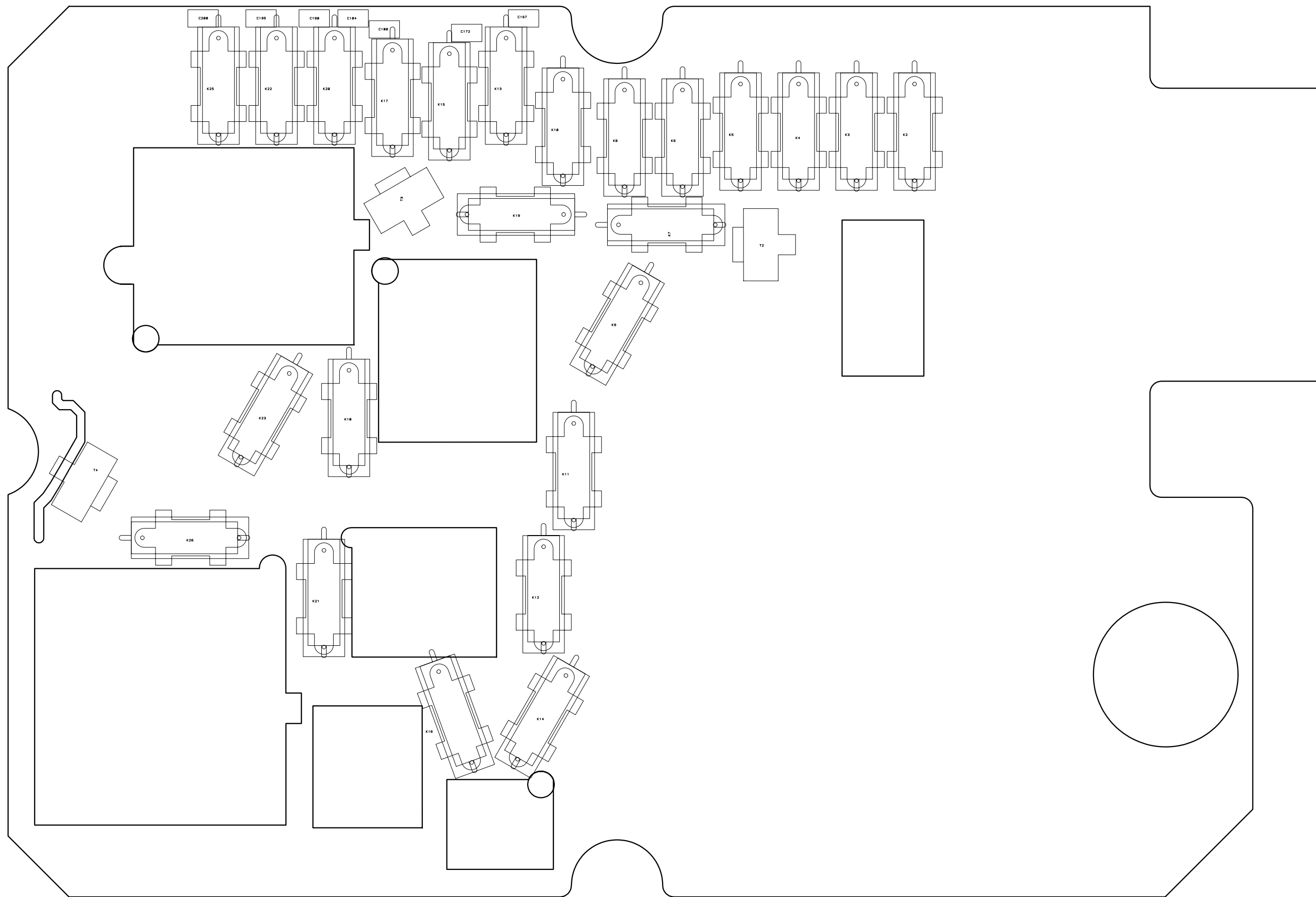
ANTENNA TUNING UNIT 945 5-5-34123B VIEWED FROM BOTTOM SIDE
