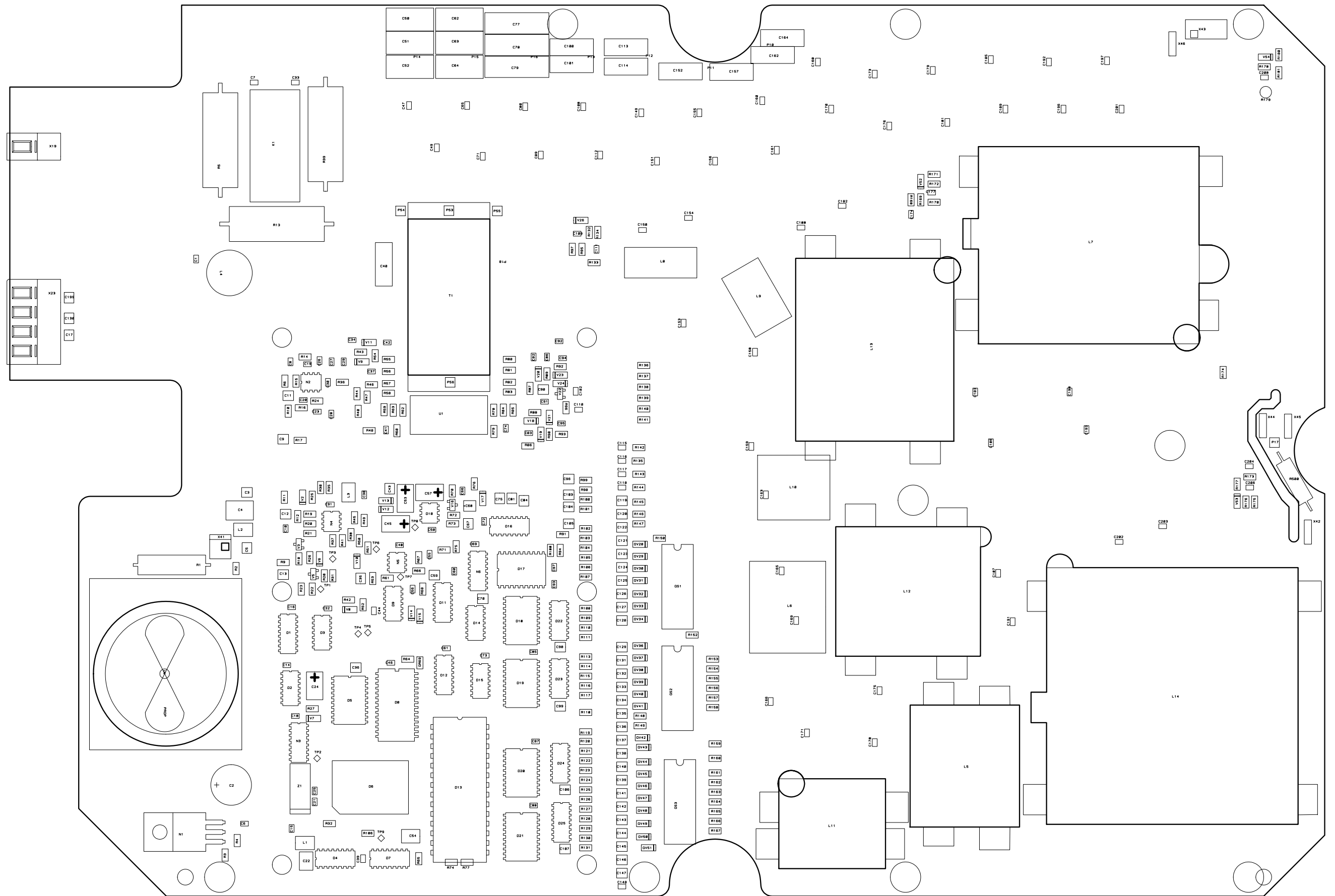
ATU BOARD 945 5-6-34123 B VIEWED FROM TOP SIDE
