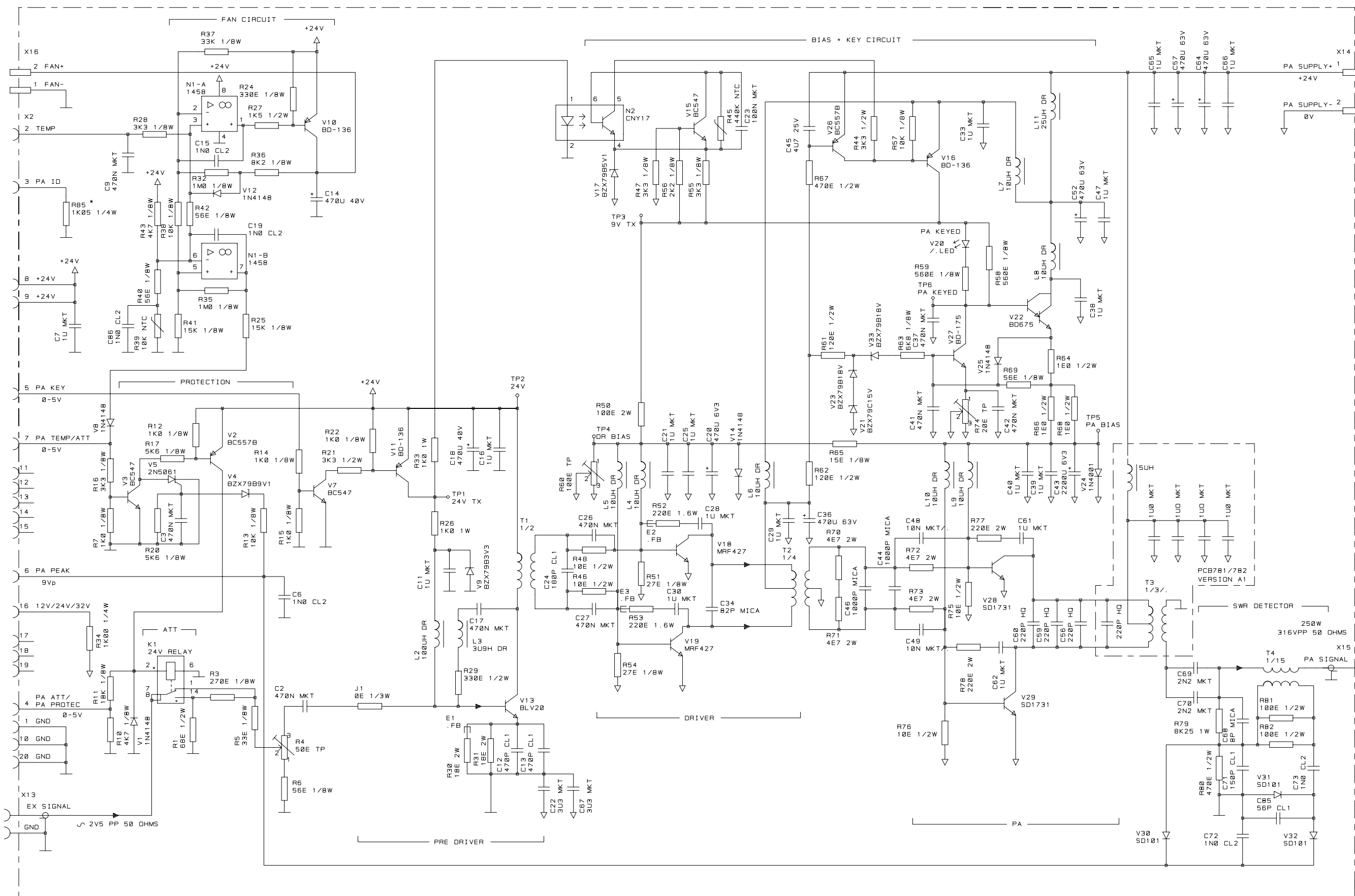
POWER AMPLIFIER 721 DIA 9938721x B4
