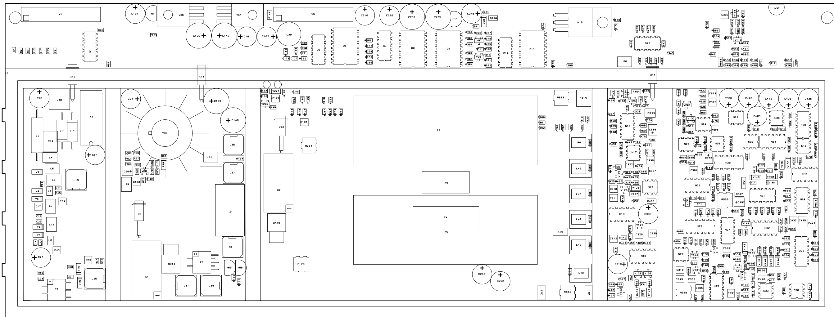
RX/EX SIGNAL PATH 715 5-6-31945 F VIEWED FROM TOP SIDE
