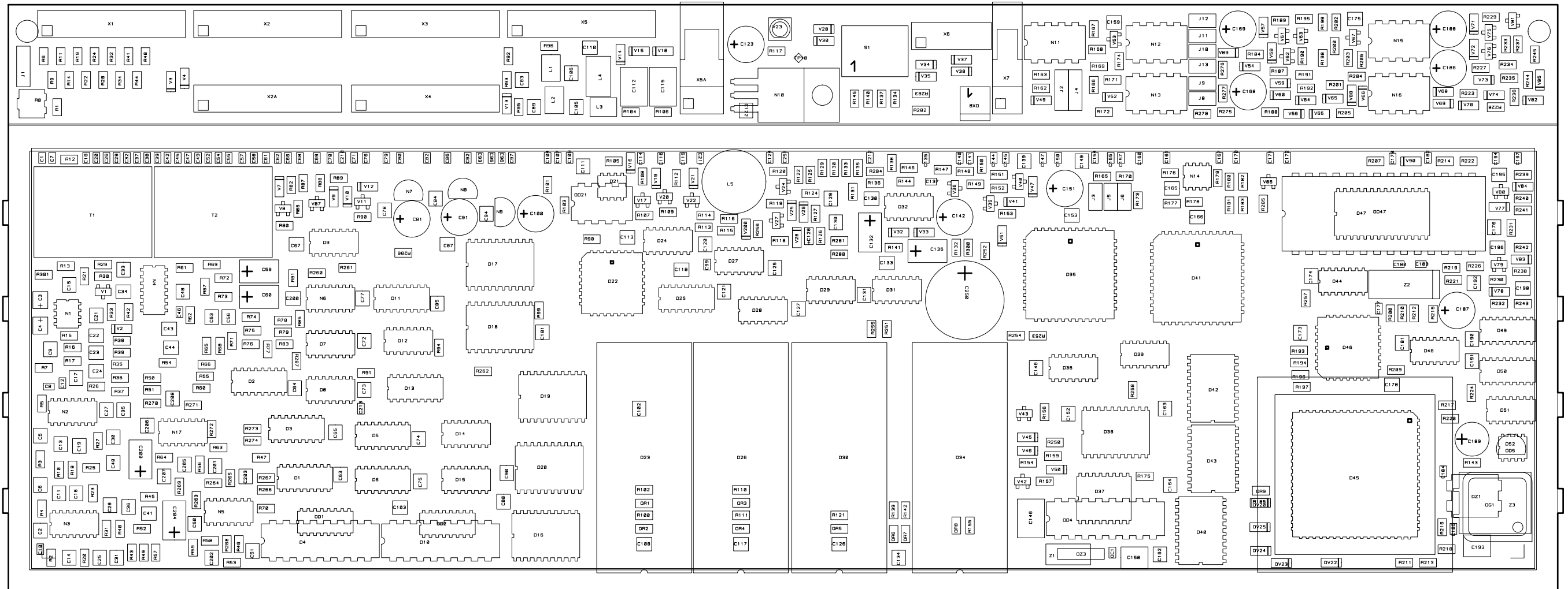
PCP BOARD 717 5-6-30309 J VIEWED FROM TOP SIDE
