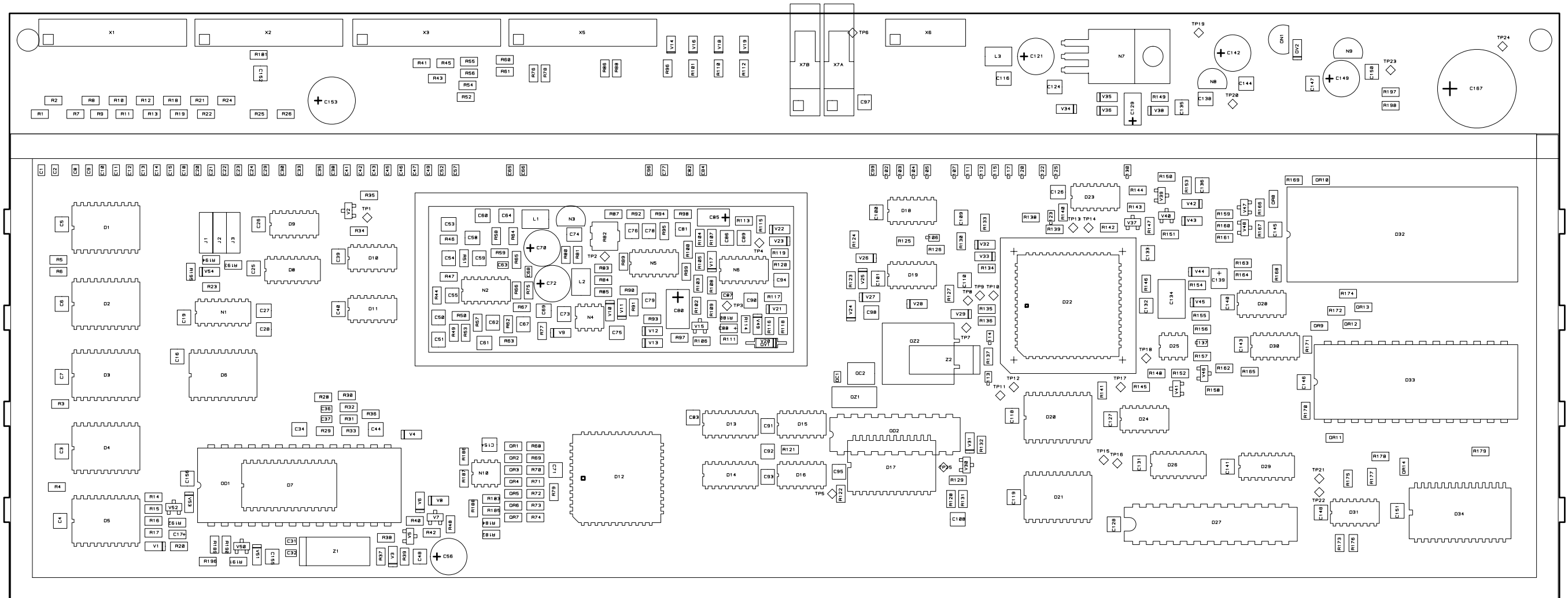
TU CONTROL BOARD 910 5-6-30818 D VIEWED FROM TOP SIDE
