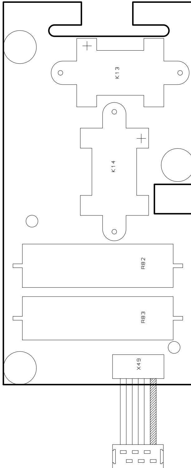
DUMMY LOAD BOARD 741 99387411 A5 VIEWED FROM TOP SIDE
