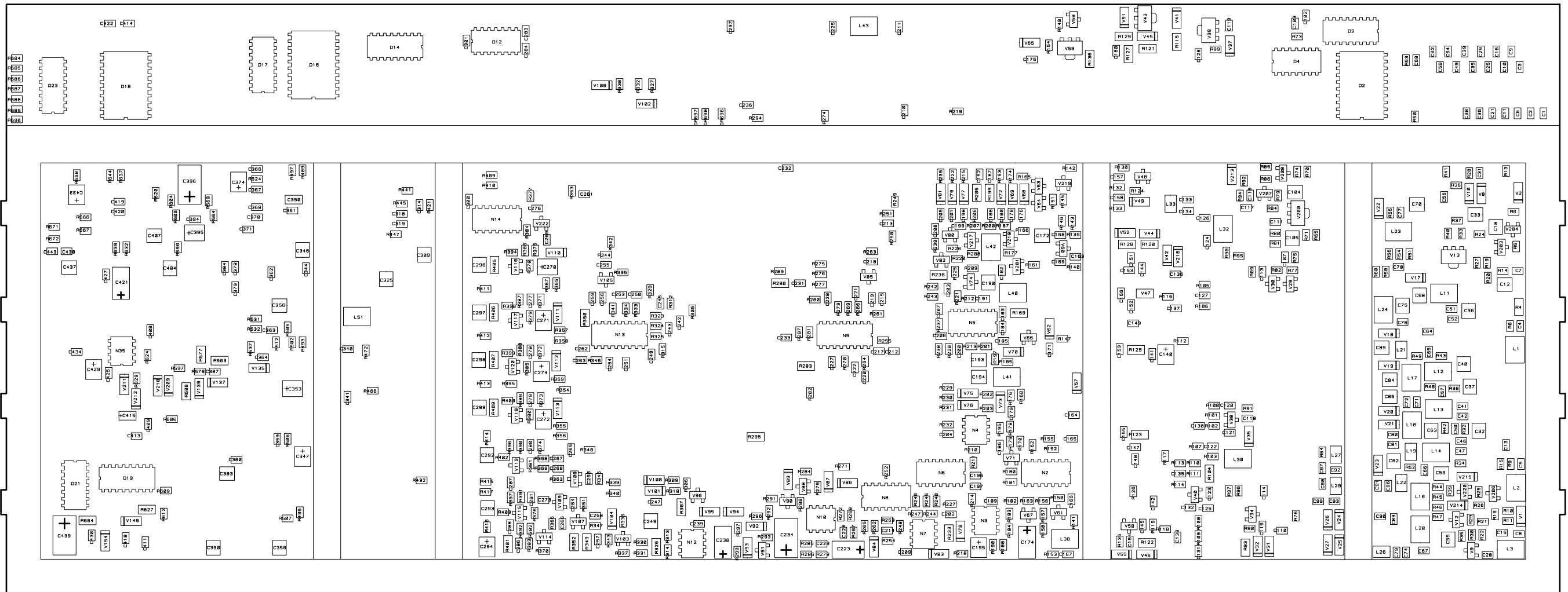
RX/EX SIGNAL PATH 715 5-5-31945 F VIEWED FROM BOTTOM SIDE
