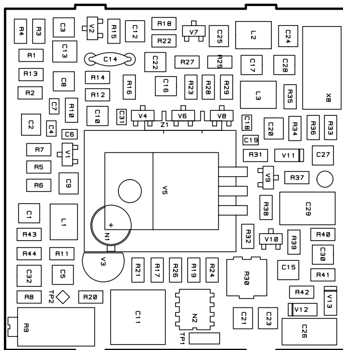
MASTER OSCILLATOR 712 / 713 / 714 / 913 5-6-30301D VIEWED FROM TOP SIDE
