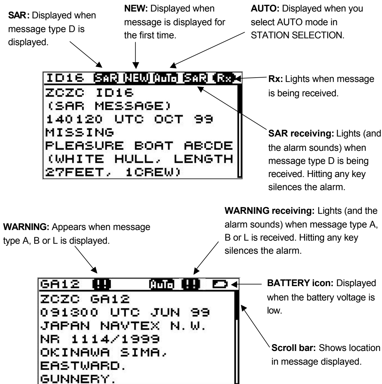
Figure 1-2 Display indications
